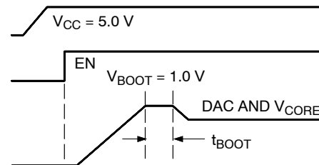
Figure 13. Power-Up Sequence for CPU
