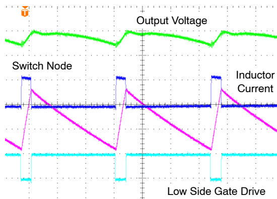
Figure 5. CCM Waveforms, 10 A Load Current
