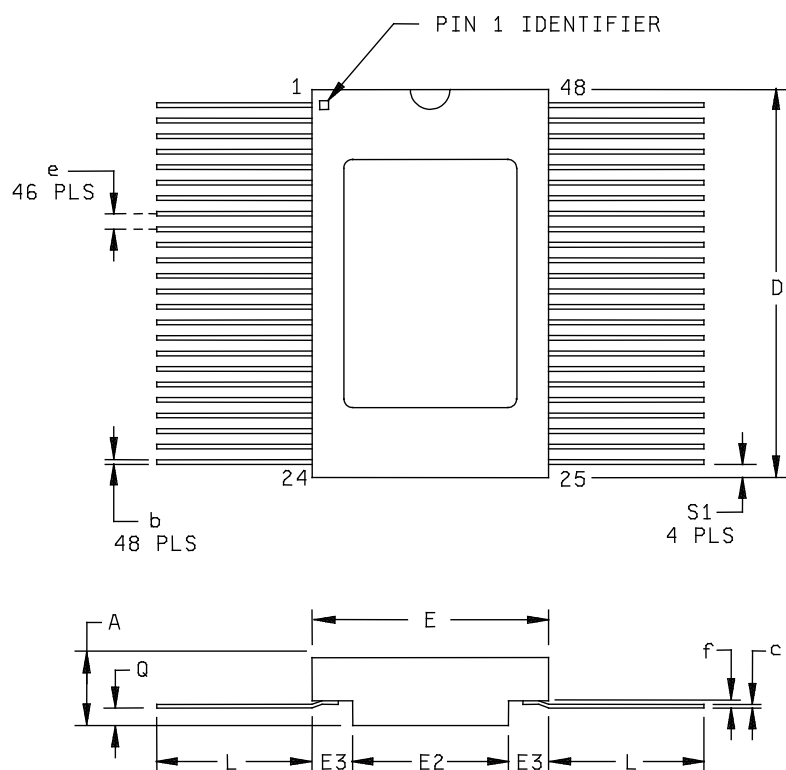
Case outline X
