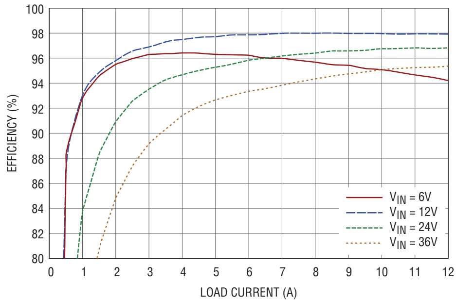
Figure 3. Efficiency vs Load Current ( V_O = 12V , CCM)
