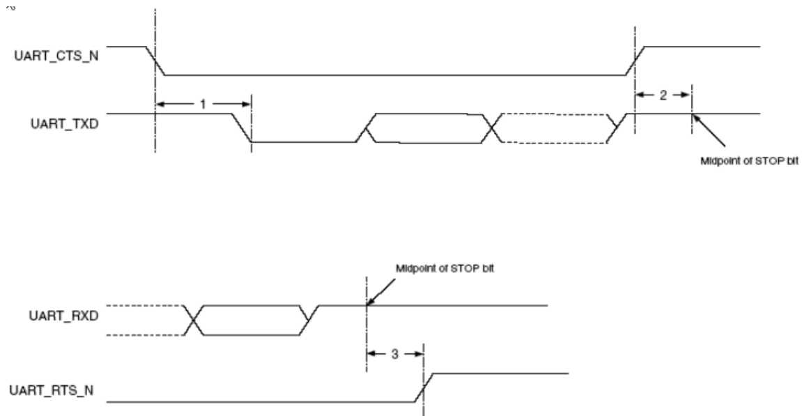
Figure 13. UART Timing
