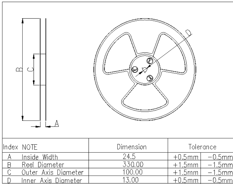
Figure 22. Reel Dimensions
