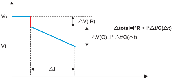
Figure 4. Voltage-time relation of capacitor unit
