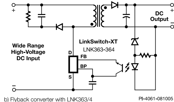
Figure 1. Typical Application with LinkSwitch-XT.
