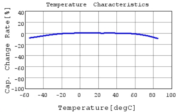
GRM033R60J225ME15 C-Temp. capchange, DC0.0V,
