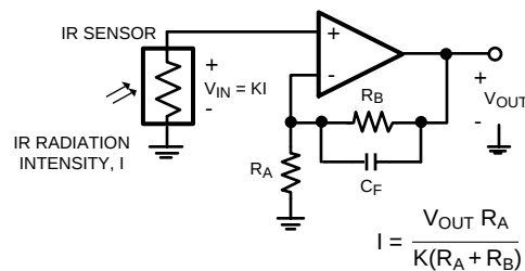
Figure 51. IR Radiation Sensor
