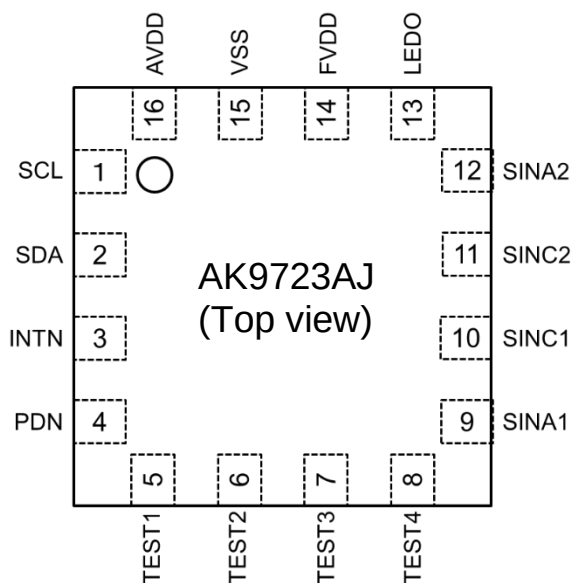
Figure 6.1 Pin Configurations
