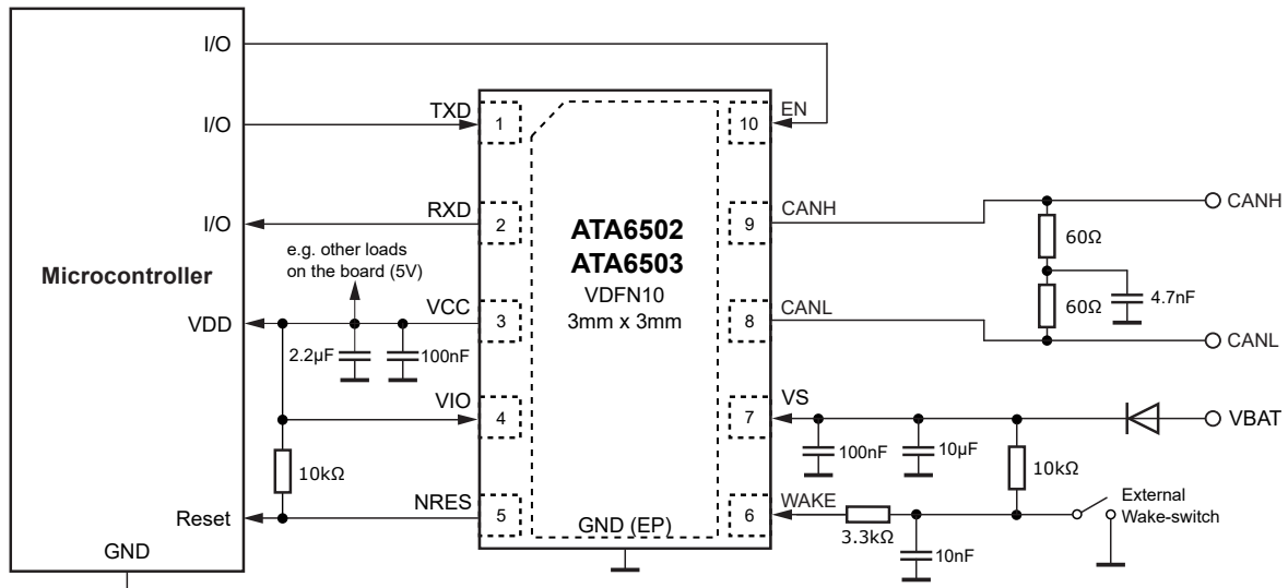
Figure 1-4. Typical Application Circuit ATA6502/ATA6503, 5V MCU
