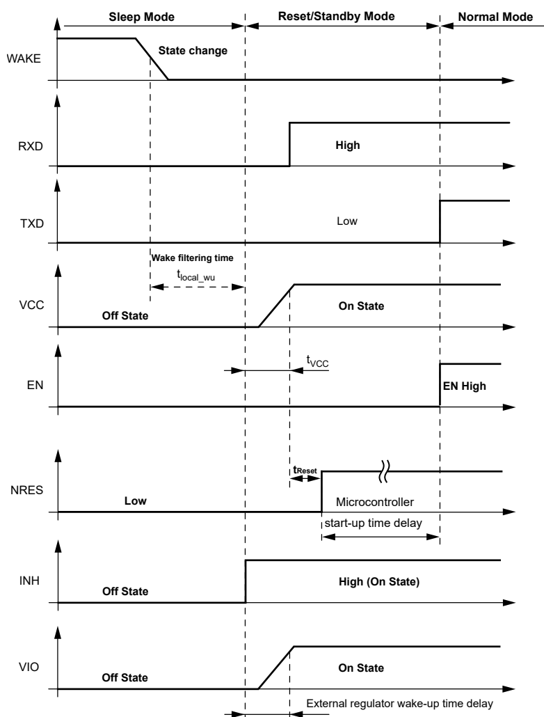
Figure 5-9. Local Wake-Up via the WAKE Pin from Sleep mode
