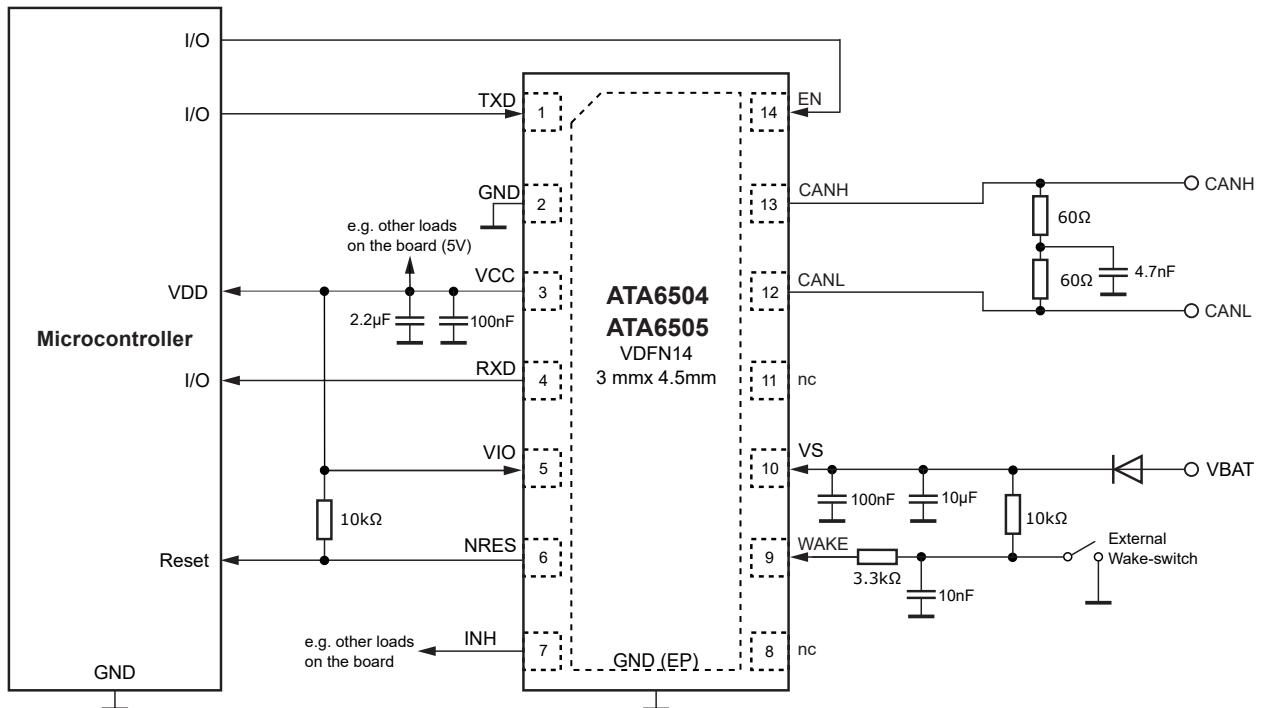
Figure 1-6. Typical Application Circuit ATA6504/ATA6505, 5V MCU
