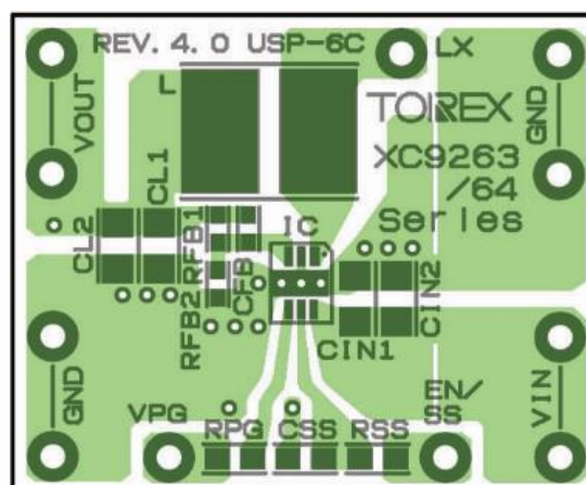
USP-6C(Front)
