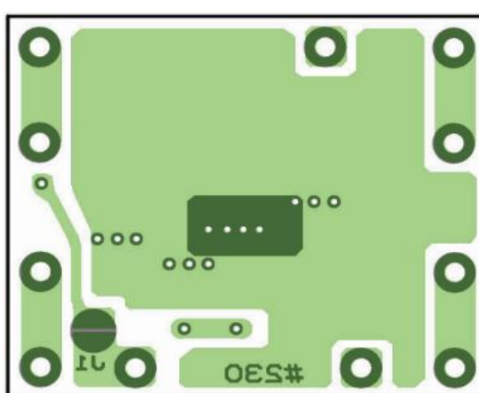
USP-6C(Back)
