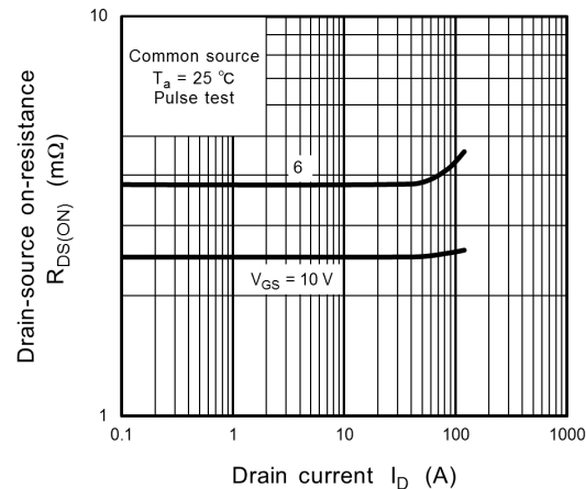
Fig. 8.8 R_{DS(ON)} - I_D
