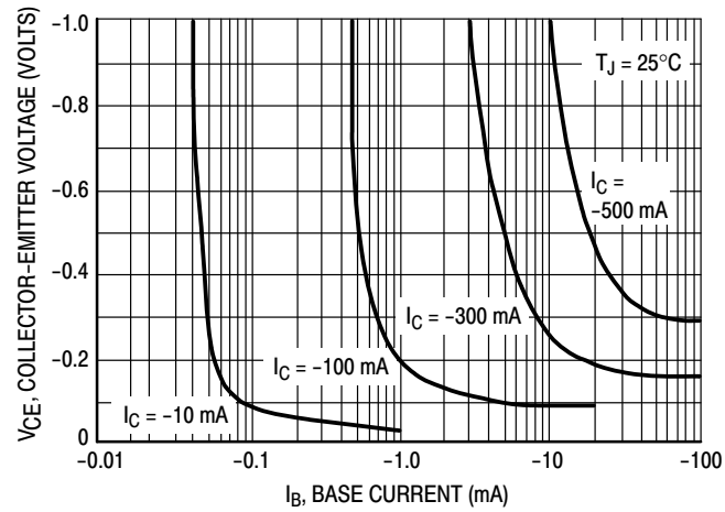
Figure 6. Saturation Region
