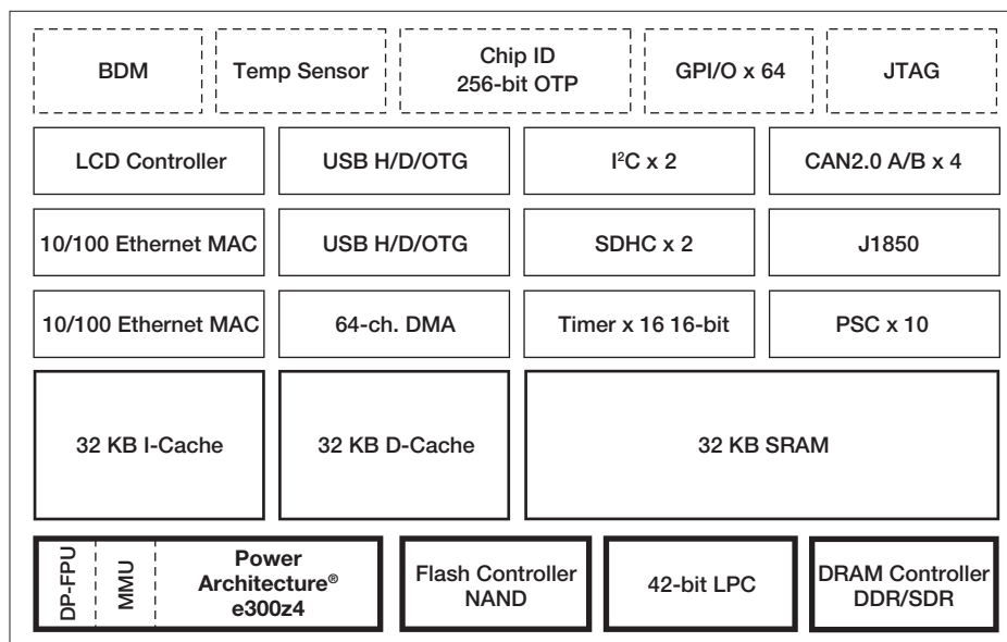
MPC5125 Block Diagram
