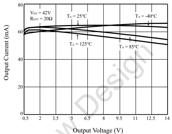
Figure 3 I_{OUT} vs. V_{OUT}
