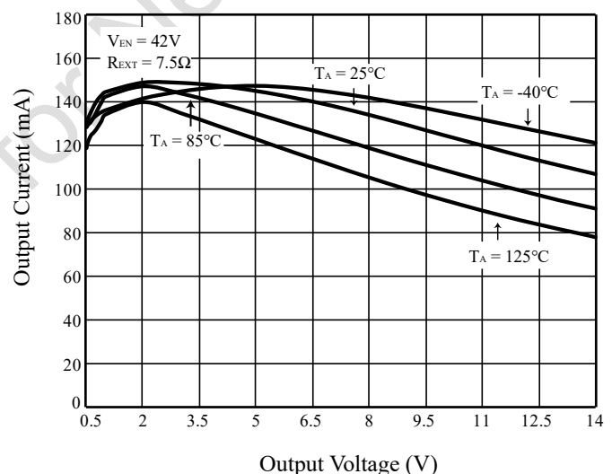
Figure 5 I_{OUT} vs. V_{OUT}
