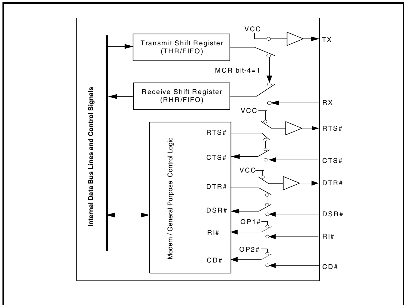
FIGURE 15. INTERNAL LOOPBACK
