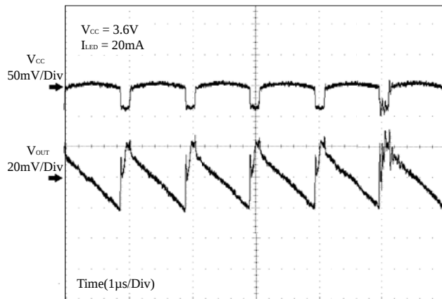
Figure 9 Ripple Voltage
