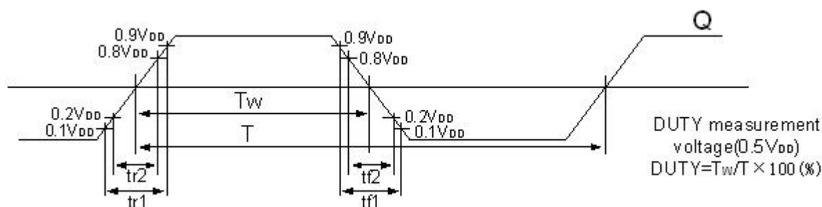
Figure1. Output switching waveform
