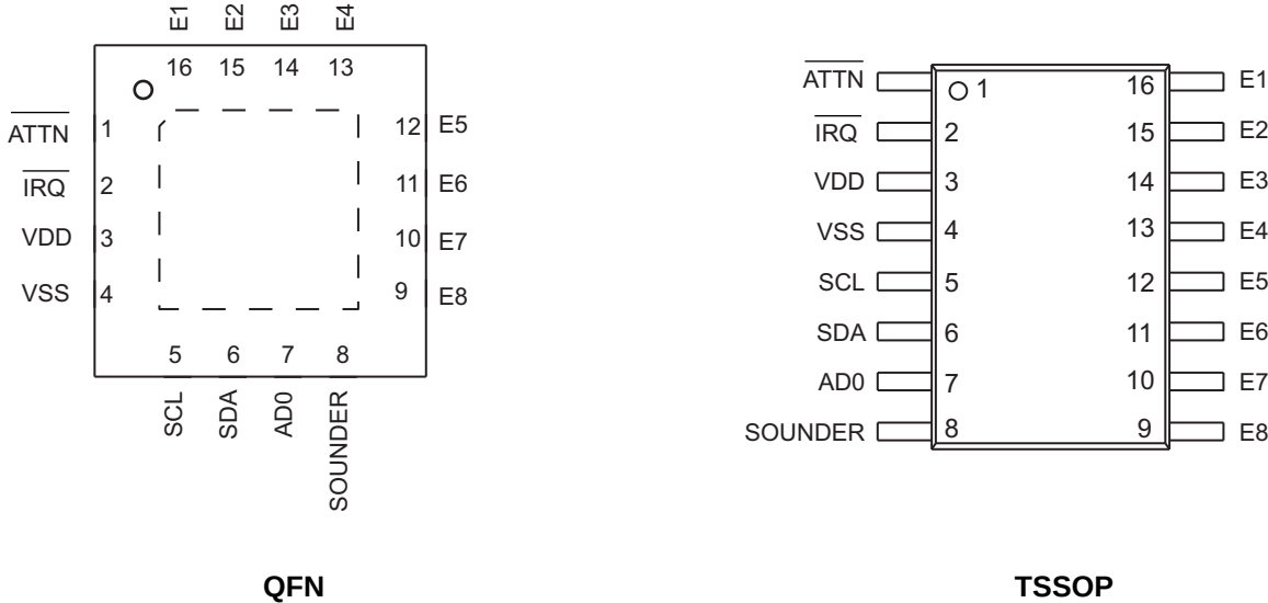
Figure 3. Package Pinouts
