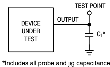
Figure 2. Test Circuit
