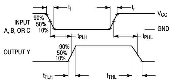
Figure 1. Switching Waveforms
