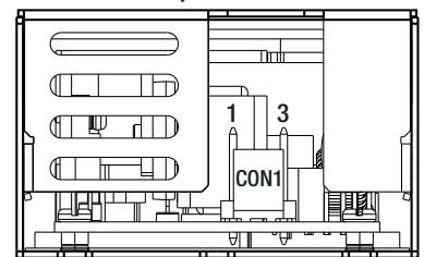
AC Input Side View
