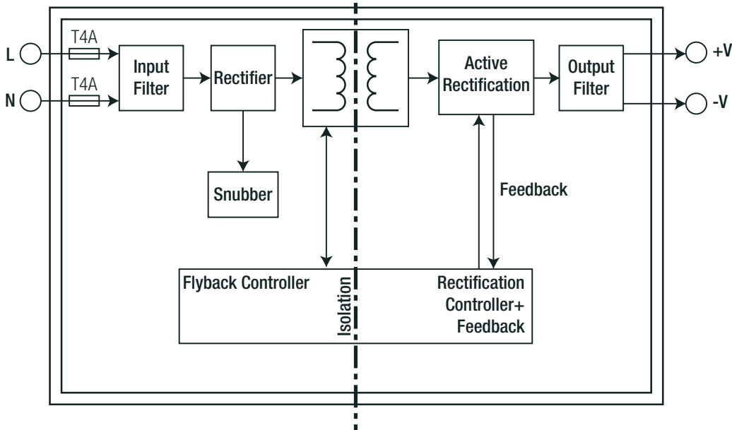
Blockdiagram (“/ENC”)
