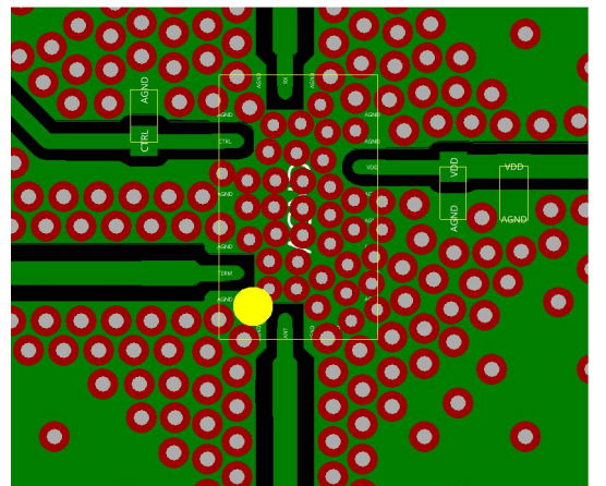
Figure 19. PCB Routings
