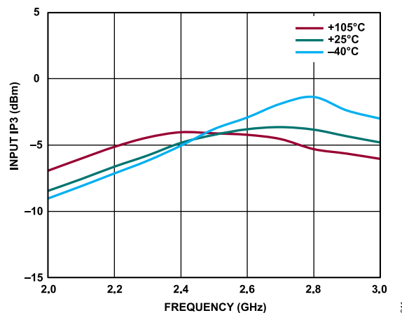
Figure 11. Input IP3 vs. Frequency at Various Temperatures
