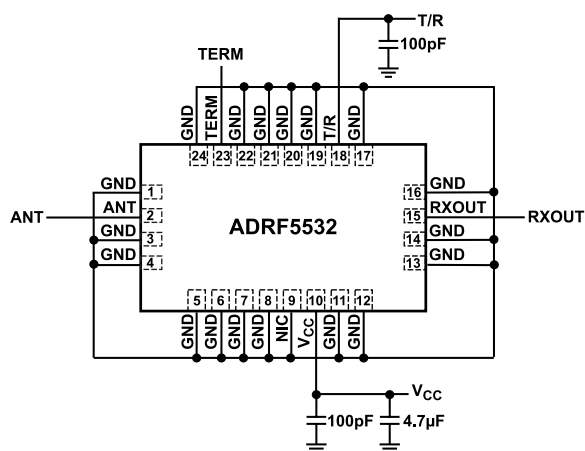
Figure 17. Recommended Schematic
