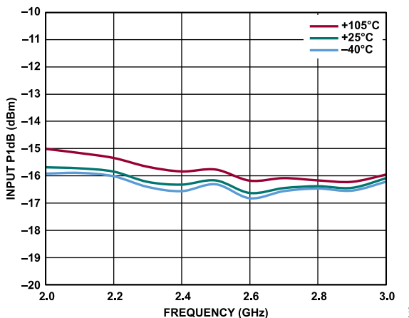
Figure 10. Input P1dB vs. Frequency at Various Temperatures
