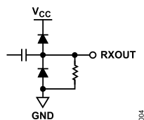
Figure 4. RXOUT Interface Schematic
