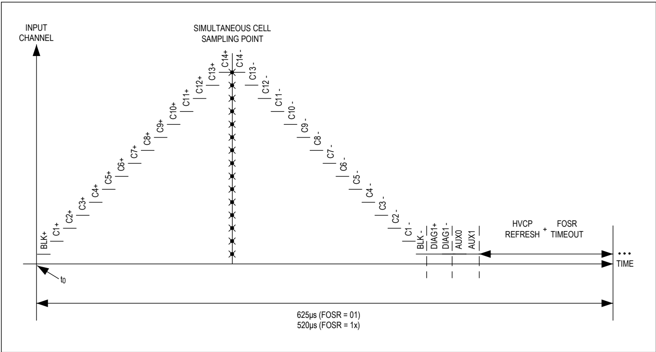
Figure 19. Acquisition - SCANCFG = 0h, SCANMODE = 0, OVSAMPL > 0h, ALTMUXSEL = 0, BLOCKEN = 1, DIAGSEL1 > 0h, AUXEN = 03h, FOSR > 0h
