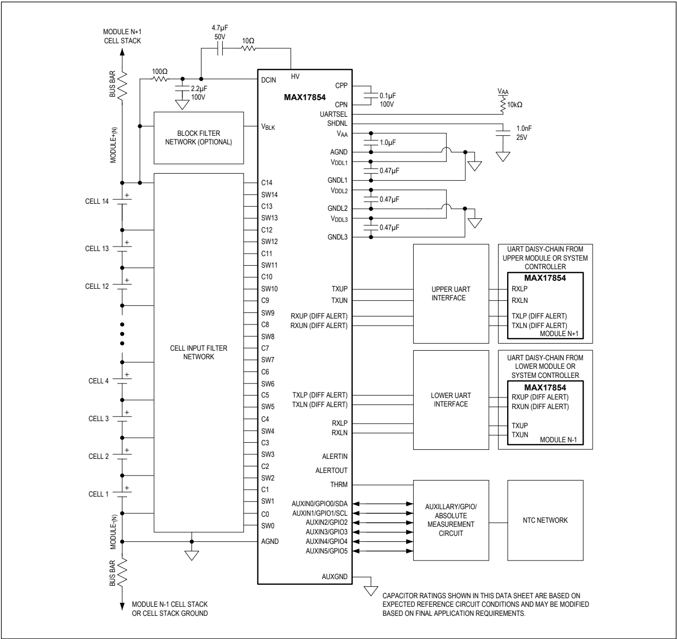
Figure 116. Simplified Application Diagram with Differential Alert Interface
