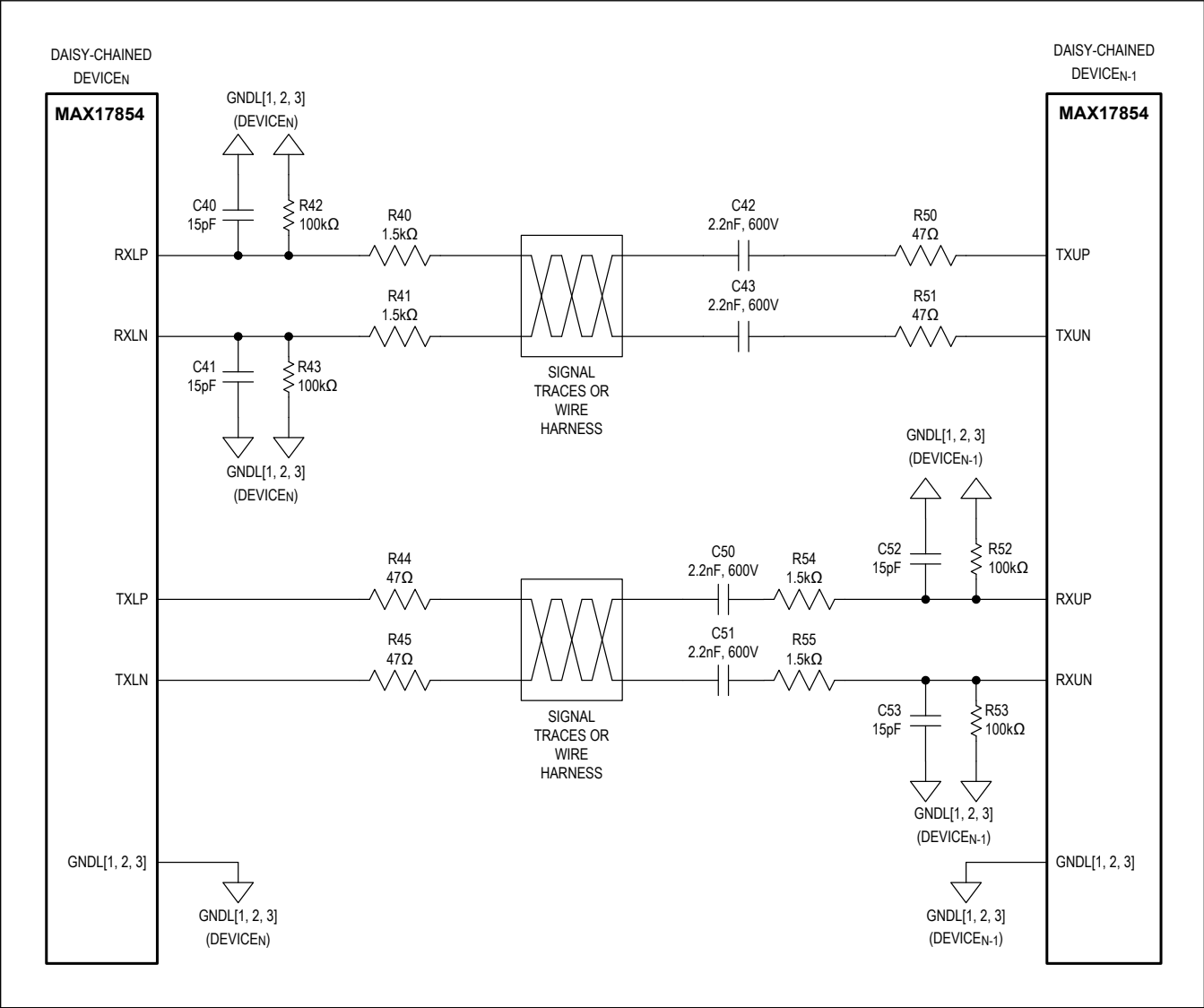
Figure 101. UART Connection
