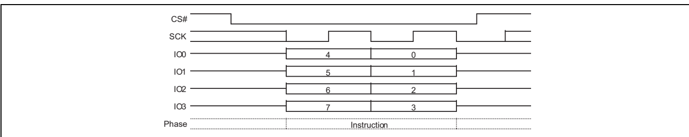
Figure 112 DPD command sequence QPI mode
