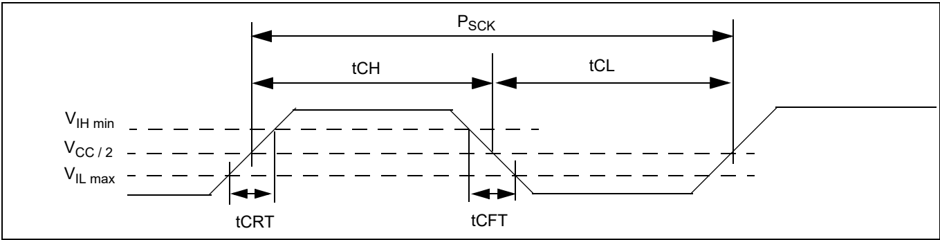
Figure 31 Clock timing
