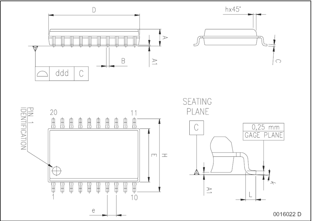
Figure 7. Package dimensions
