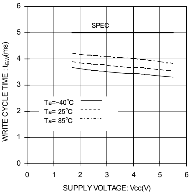
Figure 33. Write Cycle Time vs Supply Voltage
