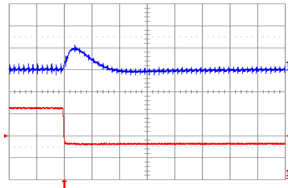
Fig. 1.5V.7: Output voltage response for V_{out} = 1.5 V to negative load current step change from 16 A to 8 A with slew rate of -5 A/ \mu s at V_{in} = 12 V. Top trace: output voltage (200 mV/div.); Bottom trace: load current (5 A/div.). C_o = 100 \mu F ceramic. Time scale: 20 \mu s/div.
