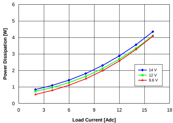
Fig. 2.5V.3: Power loss vs. load current and input voltage for V_{out} = 2.5\text{ V} converter mounted vertically with air flowing at a rate of 200\text{ LFM} ( 1\text{ m/s} ) and T_a = 25\text{ }^{\circ}\text{C} .
