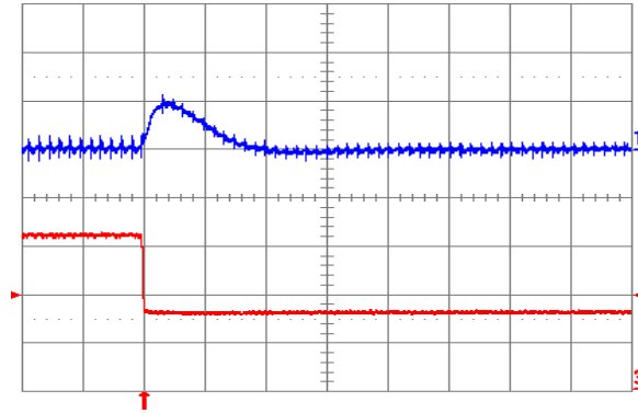
Fig. 1.8V.7: Output voltage response for V_{out} = 1.8\text{ V} to negative load current step change from 16 A to 8 A with slew rate of -5\text{ A}/\mu\text{s} at V_{in} = 12\text{ V} . Top trace: output voltage (200 mV/div.); Bottom trace: load current (5 A/div.). C_o = 100\text{ }\mu\text{F} ceramic. Time scale: 20\text{ }\mu\text{s}/\text{div.}
