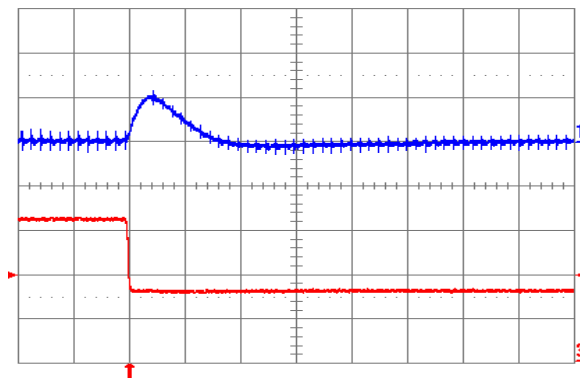
Fig. 1.2V.7: Output voltage response for V_{out} = 1.2 V to negative load current step change from 16 A to 8 A with slew rate of -5 A/ \mu s at V_{in} = 12 V. Top trace: output voltage (200 mV/div.); Bottom trace: load current (5 A/div.). C_o = 100 \mu F ceramic. Time scale: 20 \mu s/div.
