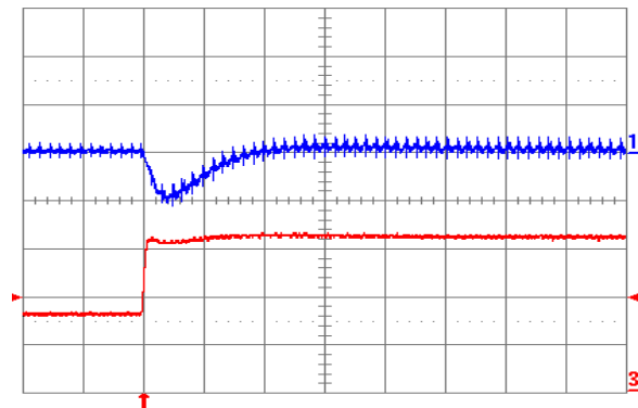
Fig. 1.8V.6: Output voltage response for V_{out} = 1.8 V to positive load current step change from 8 A to 16 A with slew rate of 5 A/μs at V_{in} = 12 V. Top trace: output voltage (200 mV/div.); Bottom trace: load current (5 A/div.). C_o = 100 \mu\text{F} ceramic. Time scale: 20 μs/div.
