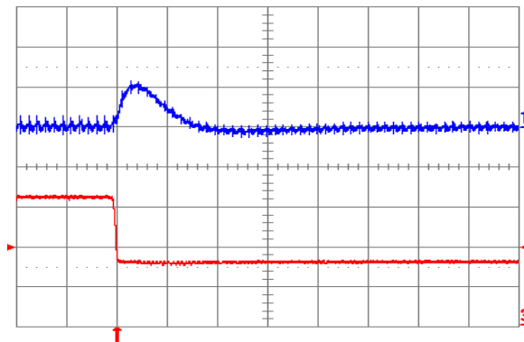
Fig. 2.5V.7: Output voltage response for V_{out} = 2.5 V to negative load current step change from 16 A to 8 A with slew rate of -5 A/ \mu s at V_{in} = 12 V. Top trace: output voltage (200 mV/div.); Bottom trace: load current (5 A/div.). C_o = 100 \mu F ceramic. Time scale: 20 \mu s/div.
