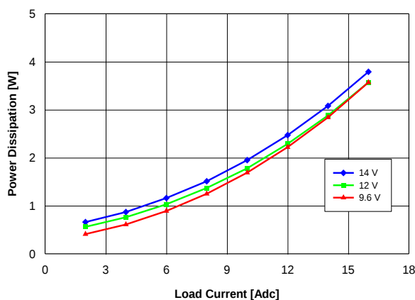
Fig. 0.7525V.3: Power loss vs. load current and input voltage for V_{out} = 0.7525\text{ V} converter mounted vertically with air flowing at a rate of 200\text{ LFM} ( 1\text{ m/s} ) and T_a = 25\text{ }^{\circ}\text{C} .
