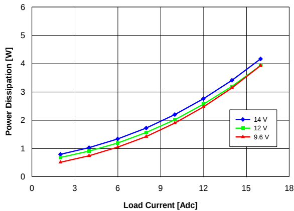
Fig. 2.0V.3: Power loss vs. load current and input voltage for V_{out} = 2.0 V converter mounted vertically with air flowing at a rate of 200 LFM (1 m/s) and T_a = 25^\circ\text{C} .
