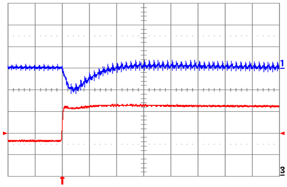
Fig. 2.0V.6: Output voltage response for V_{out} = 2.0 V to positive load current step change from 8 A to 16 A with slew rate of 5\ \text{A}/\mu\text{s} at V_{in} = 12 V. Top trace: output voltage (200 mV/div.); Bottom trace: load current (5 A/div.). C_o = 100\ \mu\text{F} ceramic. Time scale: 20\ \mu\text{s}/\text{div} .
