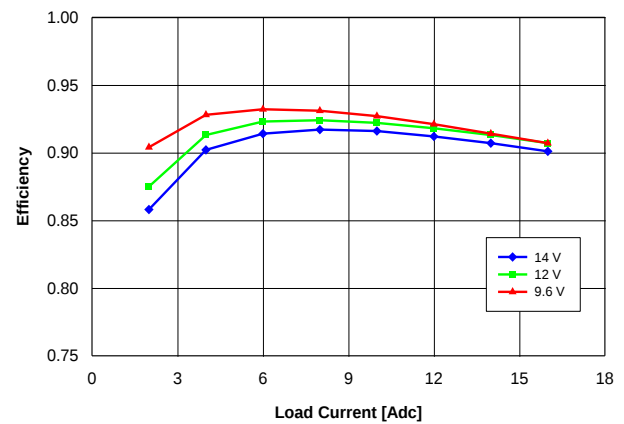
Fig. 2.5V.2: Efficiency vs. load current and input voltage for V_{out} = 2.5\text{ V} converter mounted vertically with air flowing at a rate of 200\text{ LFM} ( 1\text{ m/s} ) and T_a = 25\text{ }^{\circ}\text{C} .
