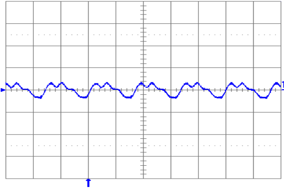
Fig. 2.5V.5: Output voltage ripple (20 mV/div.) at full rated load current into a resistive load with external capacitance 100 \mu F ceramic + 1 \mu F ceramic and V_{in} = 12 V for V_{out} = 2.5V. Time scale: 2 \mu s/div.
