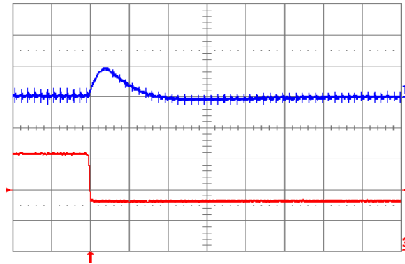
Fig. 0.7525V.7: Output voltage response for V_{out} = 0.7525 V to negative load current step change from 16 A to 8 A with slew rate of -5 A/μs at V_{in} = 12 V. Top trace: output voltage (200 mV/div.); Bottom trace: load current (5 A/div.). C_o = 100 μF ceramic. Time scale: 20 μs/div.
