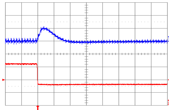
Fig. 2.0V.7: Output voltage response for V_{out} = 2.0 V to negative load current step change from 16 A to 8 A with slew rate of -5\ \text{A}/\mu\text{s} at V_{in} = 12 V. Top trace: output voltage (200 mV/div.); Bottom trace: load current (5 A/div.). C_o = 100\ \mu\text{F} ceramic. Time scale: 20\ \mu\text{s}/\text{div} .
