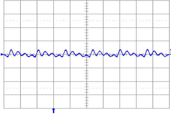
Fig. 0.7525V.5: Output voltage ripple (20 mV/div.) at full rated load current into a resistive load with external capacitance 100 μF ceramic + 1 μF ceramic and V_{in} = 12 V for V_{out} = 0.7525 V. Time scale: 2 μs/div.
