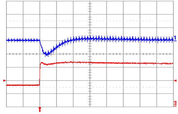
Fig. 1.5V.6: Output voltage response for V_{out} = 1.5V to positive load current step change from 8 A to 16 A with slew rate of 5 A/ \mu s at V_{in} = 12 V. Top trace: output voltage (200 mV/div.); Bottom trace: load current (5 A/div.). C_o = 100 \mu F ceramic. Time scale: 20 \mu s/div.
