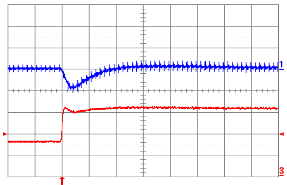
Fig. 1.0V.6: Output voltage response for V_{out} = 1.0 V to positive load current step change from 8 A to 16 A with slew rate of 5 A/μs at V_{in} = 12 V. Top trace: output voltage (200 mV/div.); Bottom trace: load current (5 A/div.). C_o = 100 \mu\text{F} ceramic. Time scale: 20 μs/div.
