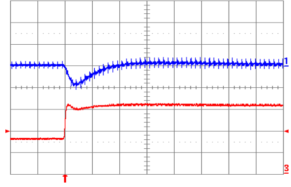
Fig. 0.7525V.6: Output voltage response for V_{out} = 0.7525 V to positive load current step change from 8 A to 16 A with slew rate of 5 A/μs at V_{in} = 12 V. Top trace: output voltage (200 mV/div.); Bottom trace: load current (5 A/div.). C_o = 100 μF ceramic. Time scale: 20 μs/div.
