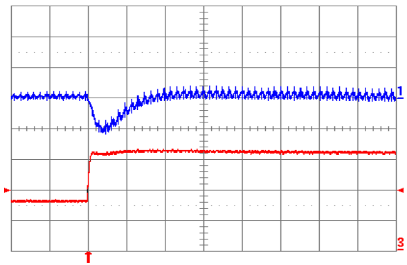
Fig. 3.3V.6: Output voltage response for V_{out} = 3.3 V to positive load current step change from 8 A to 16 A with slew rate of 5 \text{ A}/\mu\text{s} at V_{in} = 12 V. Top trace: output voltage (200 mV/div.); Bottom trace: load current (5 A/div.). C_o = 100 \mu\text{F} ceramic. Time scale: 20 µs/div.
