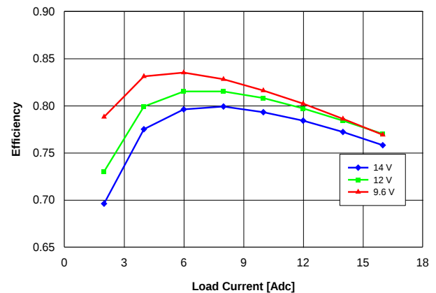
Fig. 0.7525V.2: Efficiency vs. load current and input voltage for V_{out} = 0.7525\text{ V} converter mounted vertically with air flowing at a rate of 200\text{ LFM} ( 1\text{ m/s} ) and T_a = 25\text{ }^{\circ}\text{C} .
