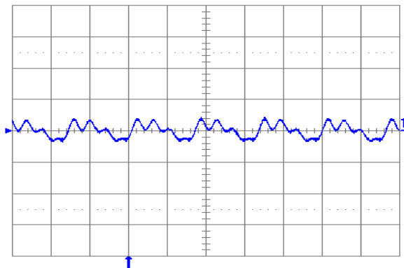
Fig. 2.0V.5: Output voltage ripple (20 mV/div.) at full rated load current into a resistive load with external capacitance 100\ \mu\text{F} ceramic + 1\ \mu\text{F} ceramic and V_{in} = 12 V for V_{out} = 2.0 V. Time scale: 2\ \mu\text{s}/\text{div} .
