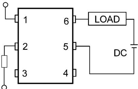
Fig. 12.2.2 B Connection
