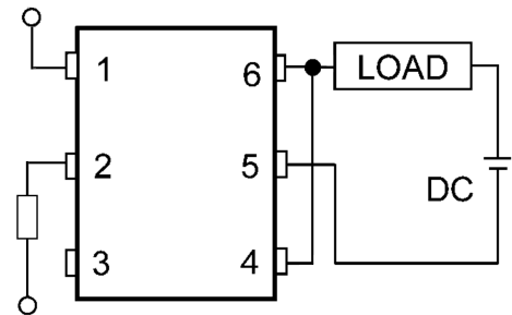
Fig. 12.2.3 C Connection
