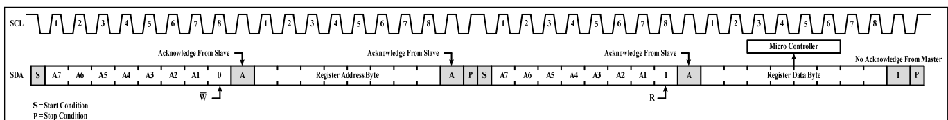
Figure 8 Reading from IS31FL3733
