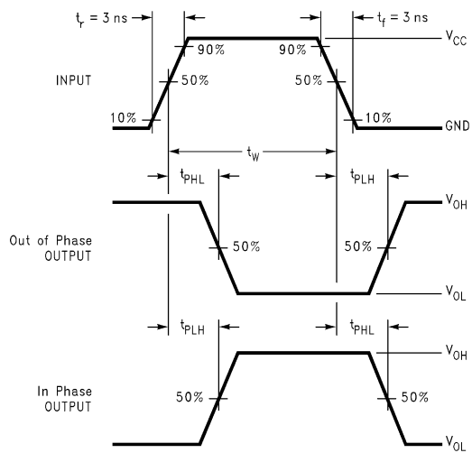
Figure 5. AC Waveforms
