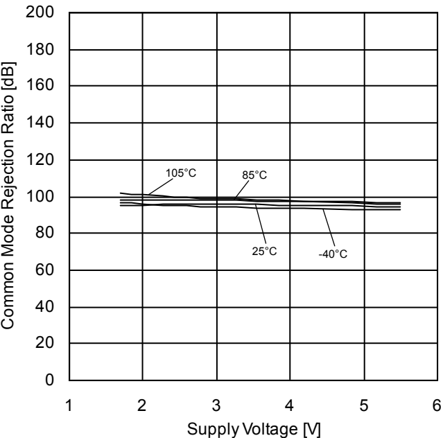
Figure 65. Common Mode Rejection Ratio vs Supply Voltage
