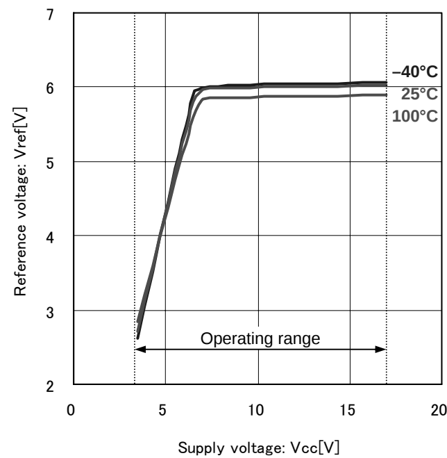
Fig.18 Reference voltage
