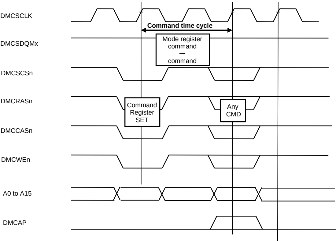
Figure 3.10.5 Example of transition from mode register write to other commands
