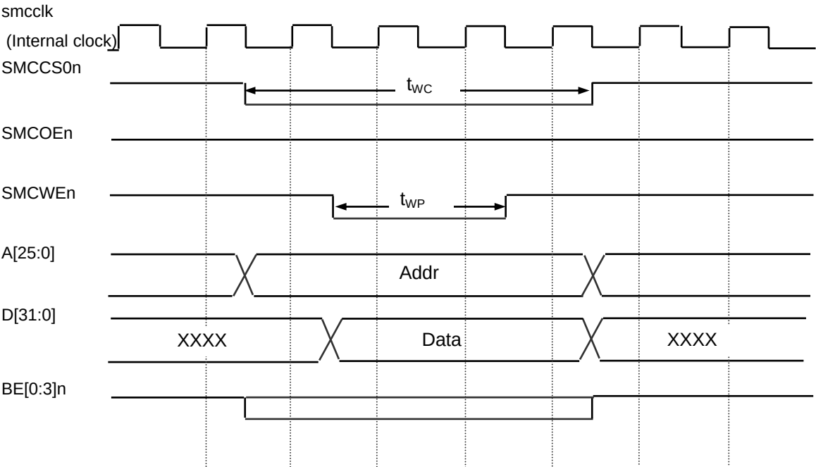
Figure 3.10.36 Asynchronous Write
