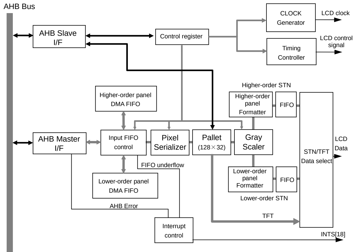
Figure 3.19.1 LCDC Block Diagram
