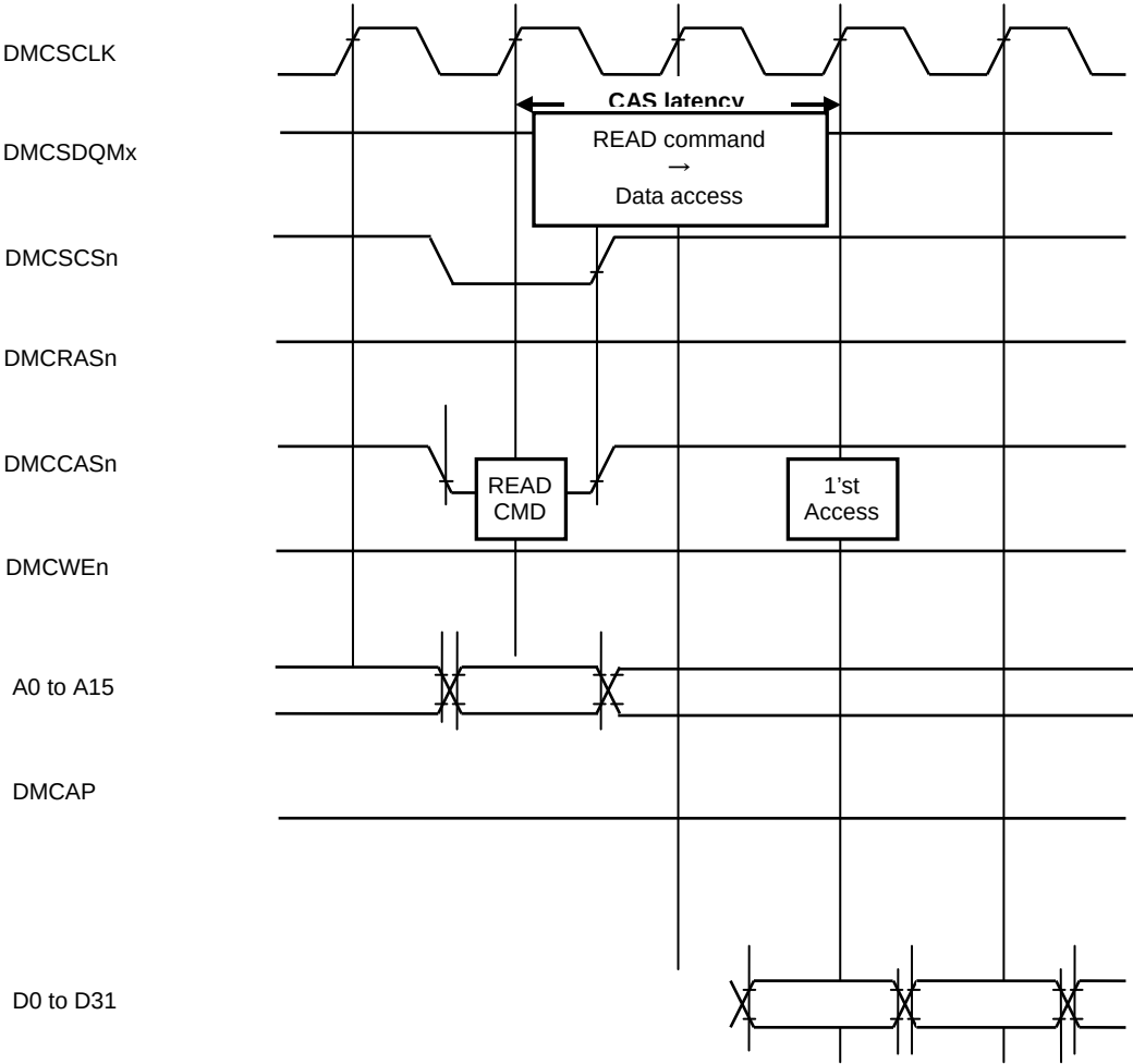
Figure 3.10.4 CAS Latency Example (CL = 2)
