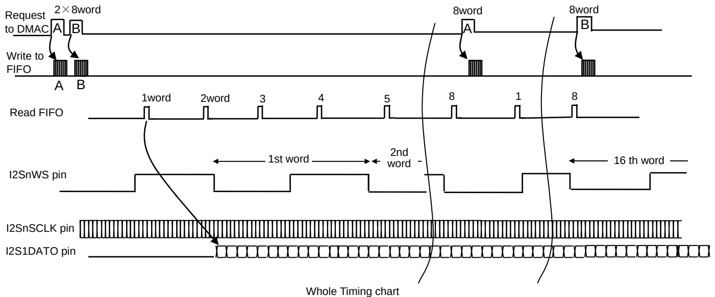
Whole Timing chart
