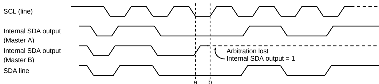
Figure 3.14.18 Arbitration lost
