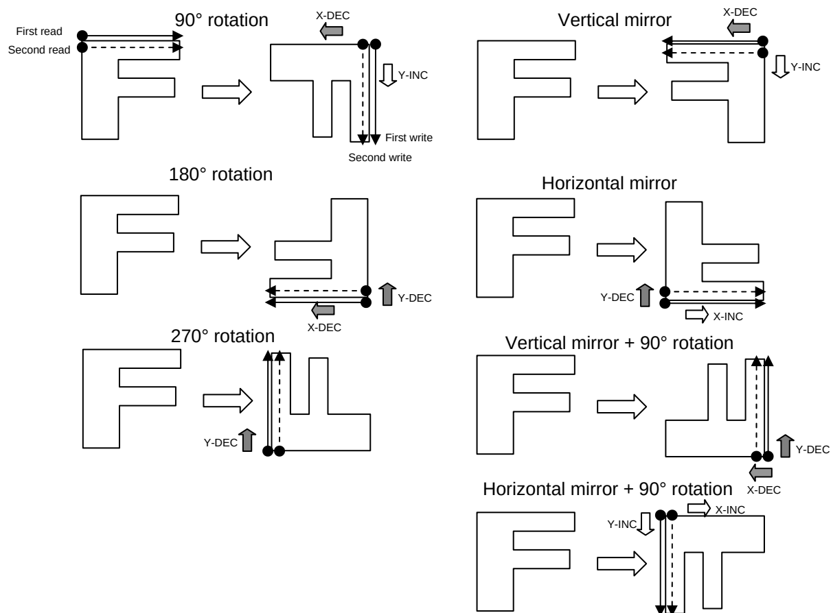
Figure 3.20.10 Rotation processing
