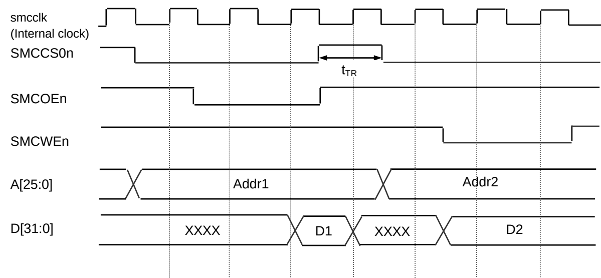
Figure 3.10.21 Asynchronous Write after Asynchronous Read
