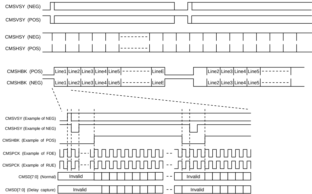
Basis timing
