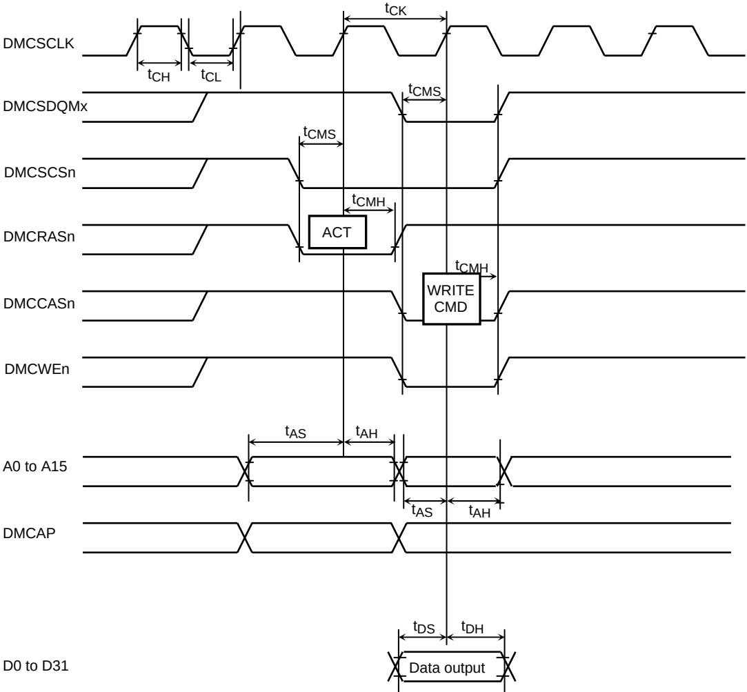
(2) SDRAM write timing
