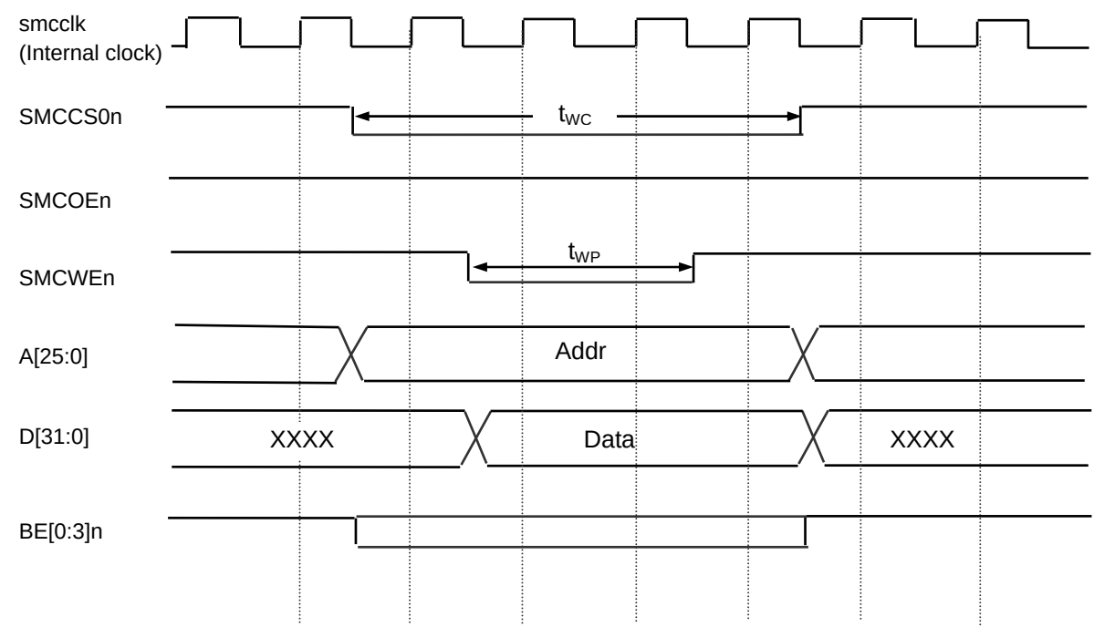
Figure 3.10.19 Asynchronous Write
