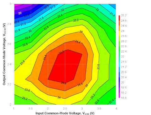
Figure 6-15. OIP3 Across V_{ICM} and V_{OCM} at 500MHz
