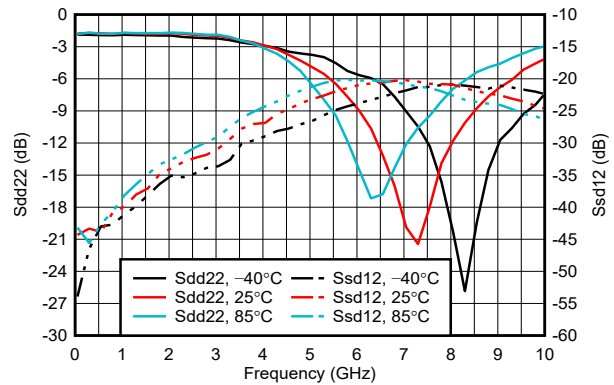
Figure 6-32. S-Parameters Across Temperature in S2D Configuration
