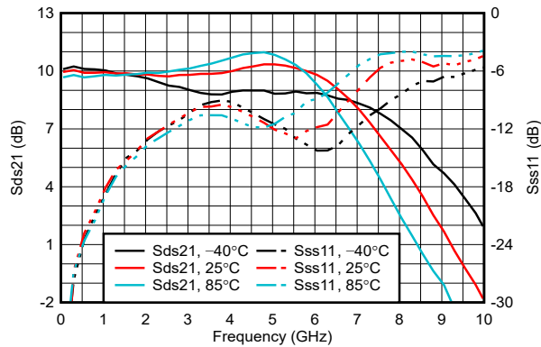
Figure 6-31. S-Parameters Across Temperature in S2D Configuration
