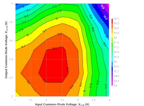
Figure 6-16. OIP3 Across V_{ICM} and V_{OCM} at 2GHz
