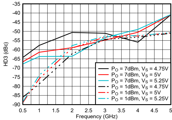
Figure 6-37. HD3 Across Supply Voltage and Output Power
