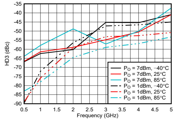
Figure 6-38. HD3 Across Temperature and Output Power
