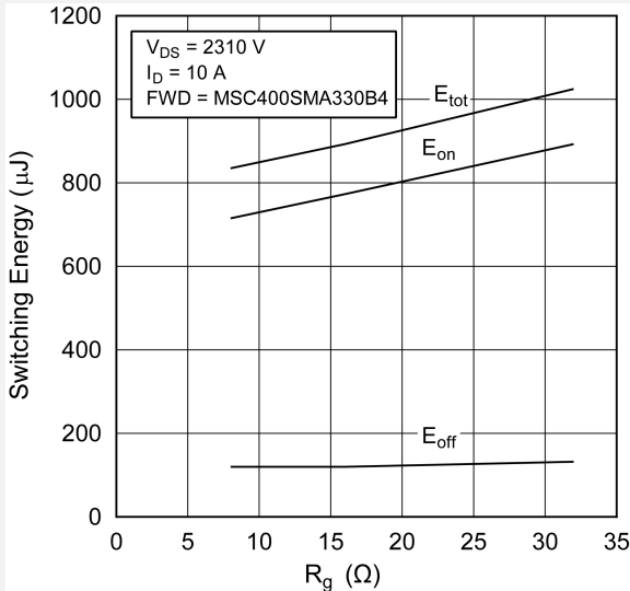
Figure 1-12. Switching Energy vs. R_g
