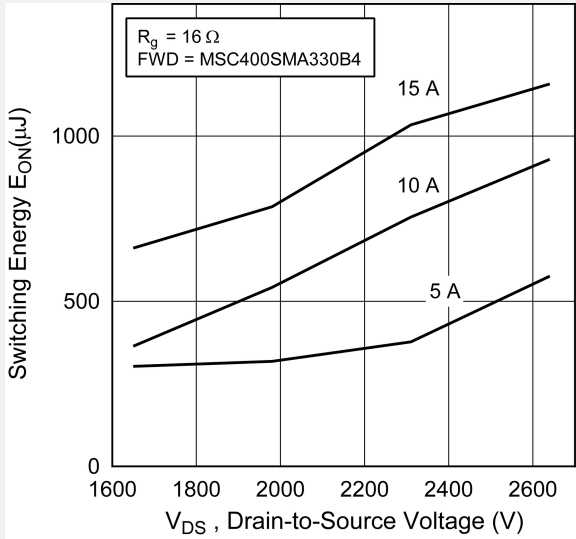
Figure 1-10. Switching Energy E_{on} vs. V_{DS} & I_D
