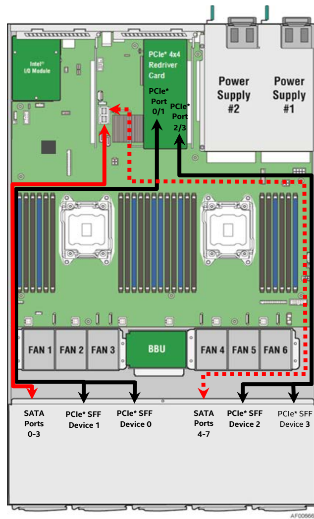
Figure 11. 1U Combo Backplane (iPC – A1U44X25NVMEDK) Cable Routing
