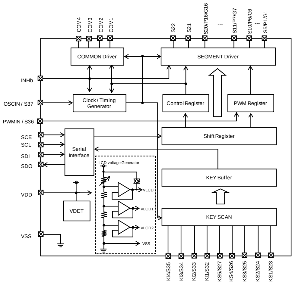
Figure 2. Block Diagram
