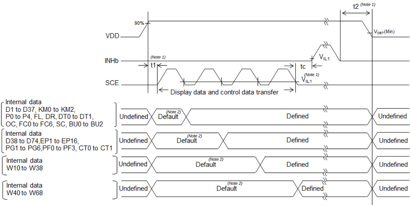
Figure 42. Power ON/OFF and INHb Control Sequence (1/2-Duty)
