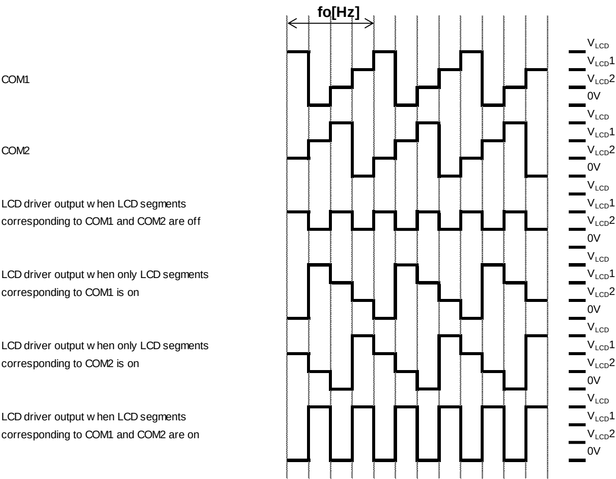
Figure 30. LCD Waveform (Line Inversion, 1/2 DUTY, 1/3 BIAS) (Note)
