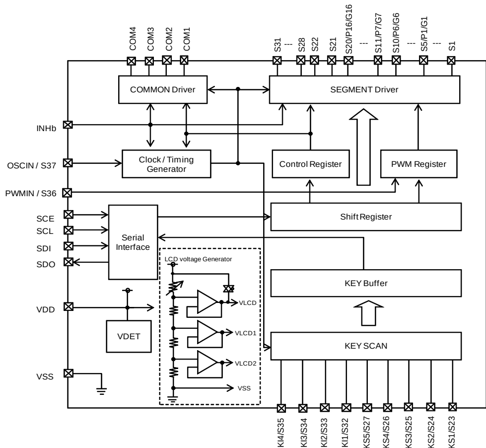
Figure 4. Block Diagram
