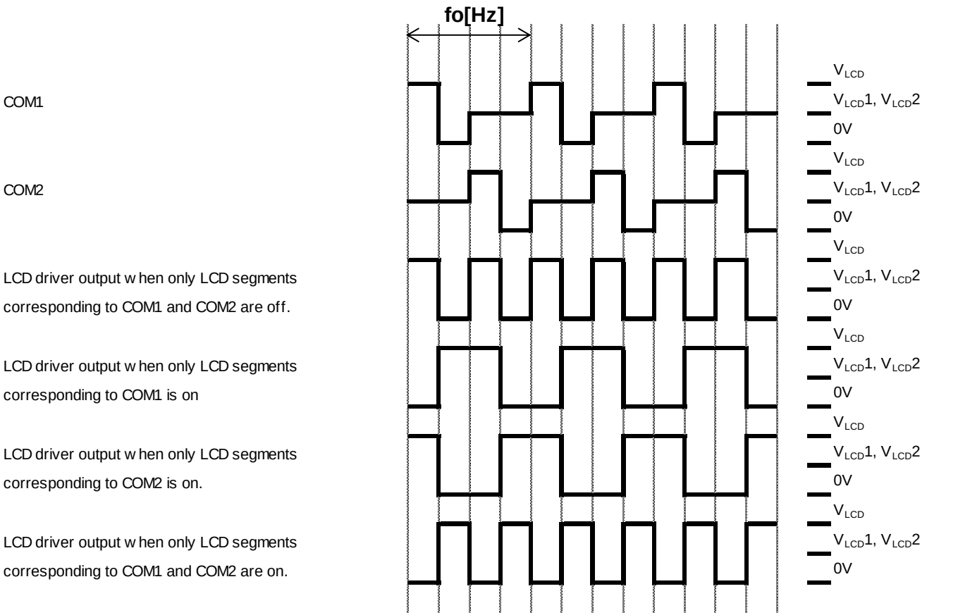
Figure 31. LCD Waveform (Line Inversion, 1/2 DUTY, 1/2BIAS) (Note)
