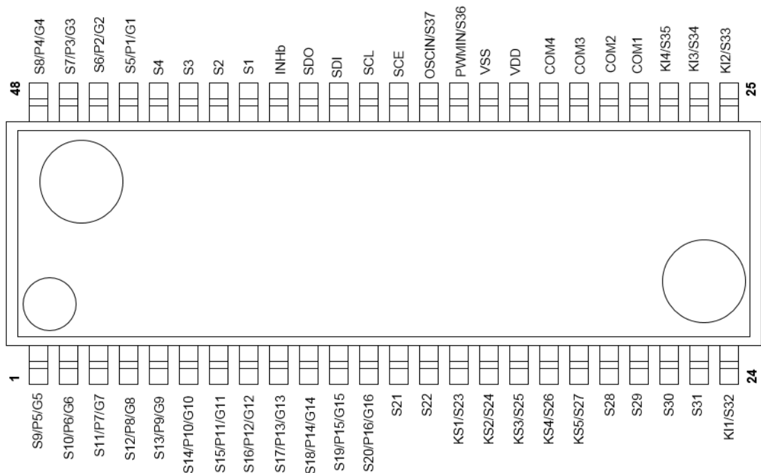
Figure 5. Pin Configuration (TOP VIEW)
