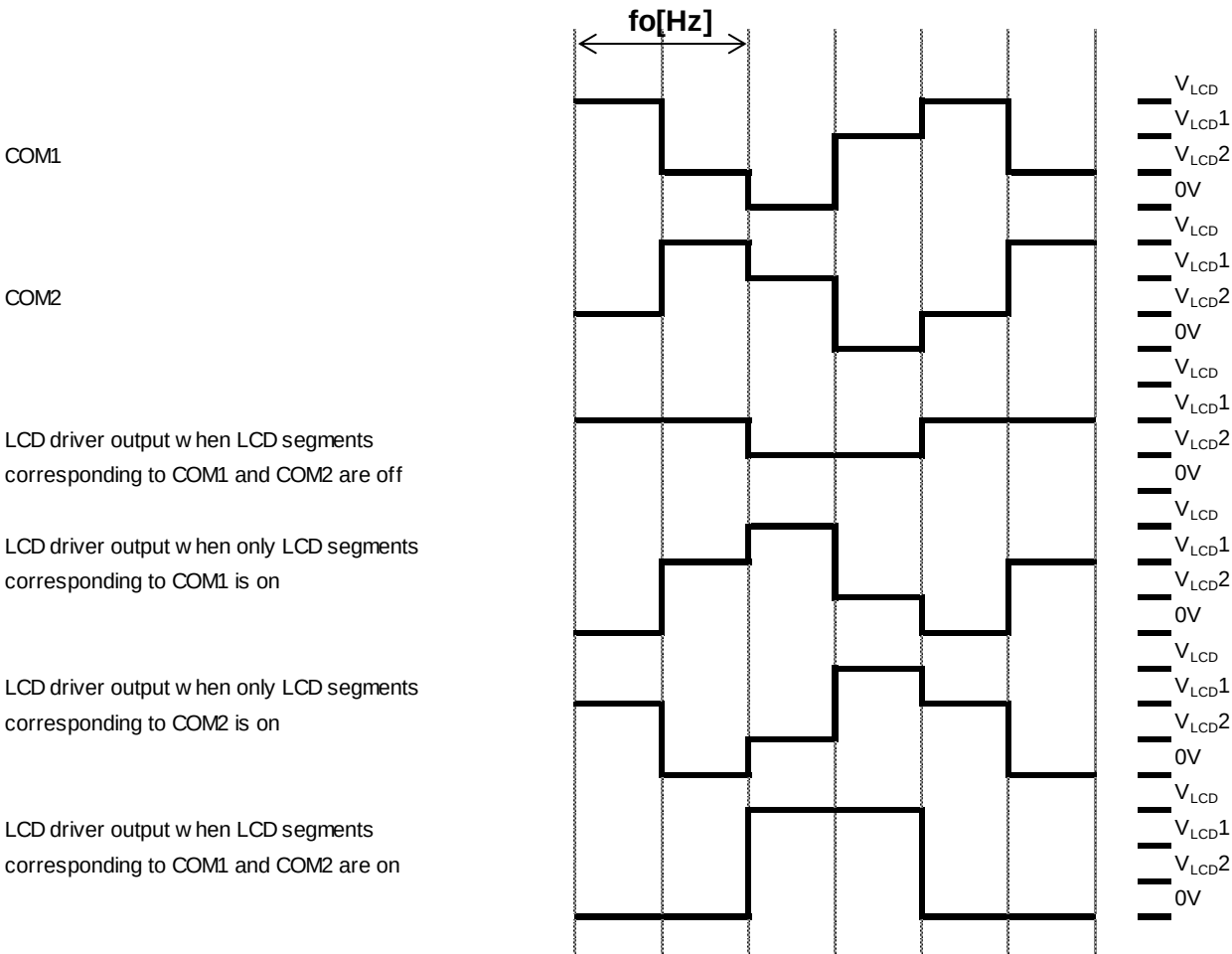
Figure 37. LCD Waveform (Frame Inversion, 1/2 DUTY, 1/3BIAS) (Note)
