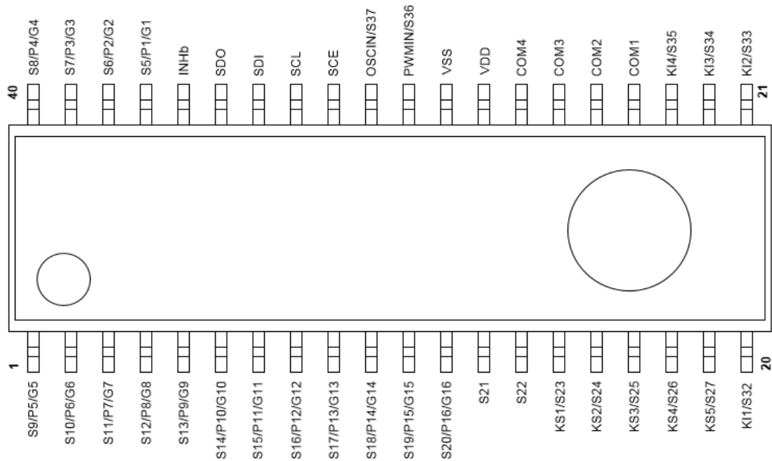
Figure 3. Pin Configuration (TOP VIEW)
