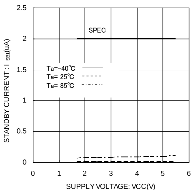
Figure 19. Standby current I_{SBI}(CS=0V, ORG=VCC \text{ or } OPEN)
