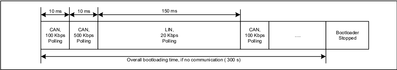
Figure 29-1 Bootloading sequence
