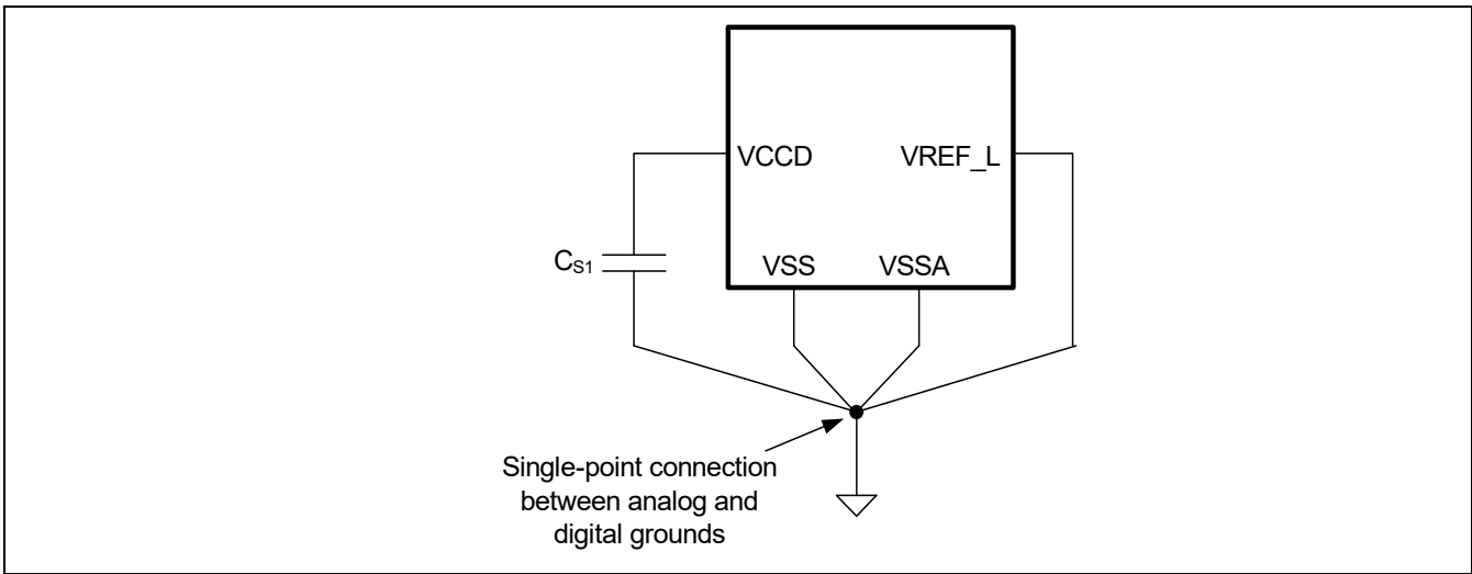
Figure 26-2 Smoothing capacitor
