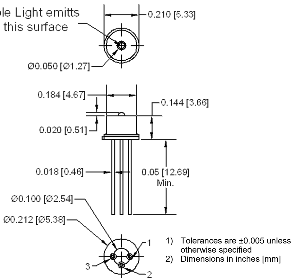
Bottom View
