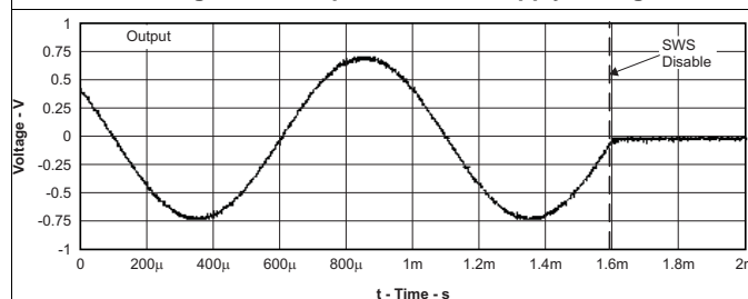
Figure 23. Shutdown Time
