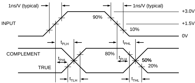
Figure 4. Propagation Delay and Transition Times
