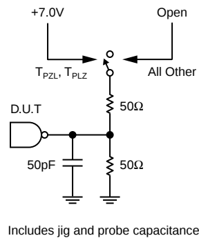
Figure 3. Test Load
