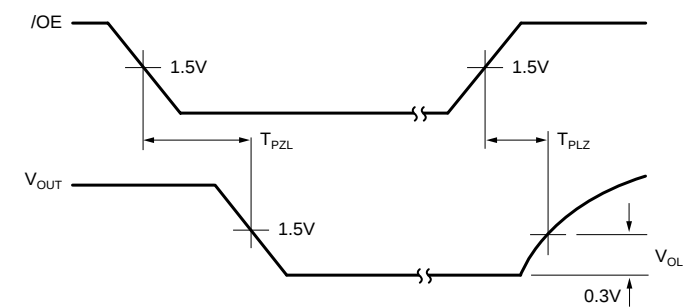
Figure 1. 3-State Output Low Enable and Disable Times
