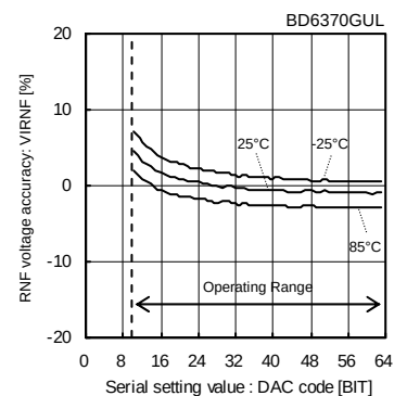
Fig.12 RNF Voltage Accuracy (Const.-Current drive block, R_{NFx}=1.0\Omega , R_L=10\Omega )
