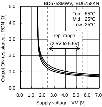
Fig.32 Output ON-Resistance (Linear Constant-Current Drive block)
