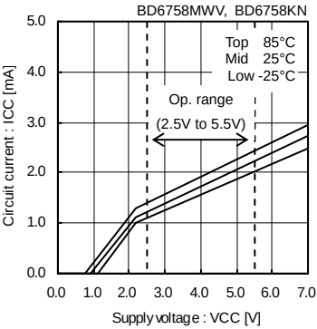
Fig.30 Circuit current
