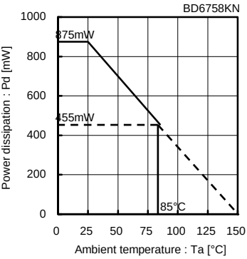
Fig.36 Power Dissipation Reduction
