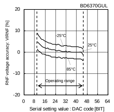
Fig.9 RNF Voltage Accuracy (Const.-Current drive block, R_{NFx}=0.5\Omega , R_L=10\Omega )
