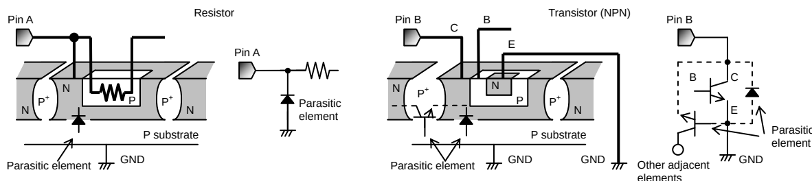
Fig.53 Example of Simple IC Architecture
