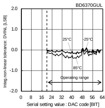
Fig.5 Integral Non-Linear Tolerance (Const.-Voltage drive block, RL=20Ω)
