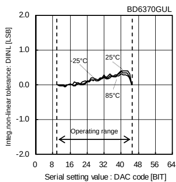
Fig.8 Integral Non-Linear Tolerance (Const.-Current drive block, R_{NFx}=0.5\Omega , R_L=10\Omega )
