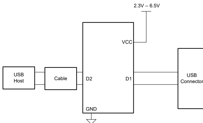
Simplified Schematic
