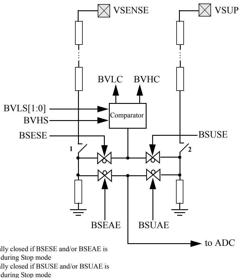
Figure 17-1. BATS Block Diagram
