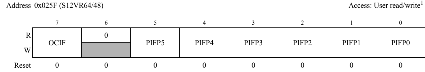
Figure 2-47. Port P Interrupt Flag Register (PIFP - S12VR64/48)
