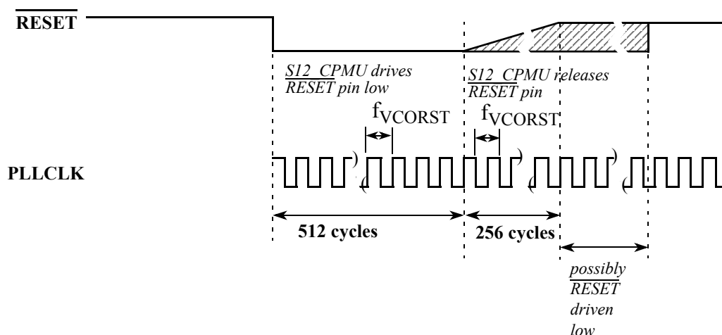
Figure 4-39. RESET Timing
