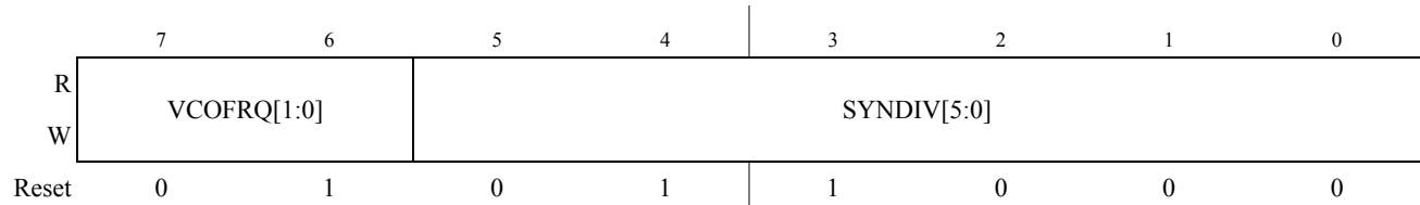
Figure 4-4. S12CPMU_UHV_V8 Synthesizer Register (CPMUSYNR)
