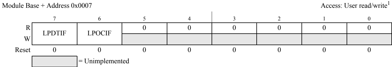
Figure 16-10. LIN Interrupt Flags Register (LPIF)
