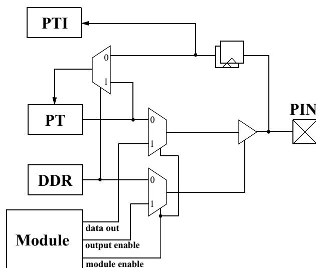
Figure 2-70. Illustration of I/O pin functionality
