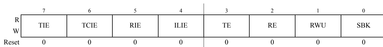
Figure 10-9. SCI Control Register 2 (SCICR2)
