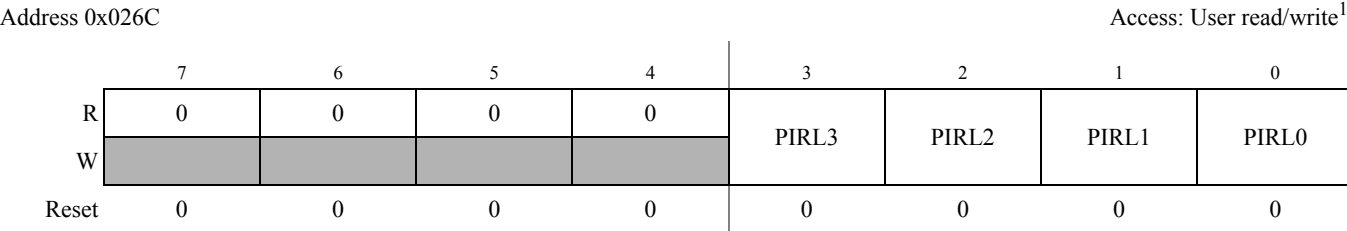
Figure 2-52. Port L Input Divider Ratio Selection Register (PIRL)
