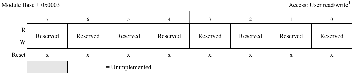
Figure 14-5. Reserved Register
