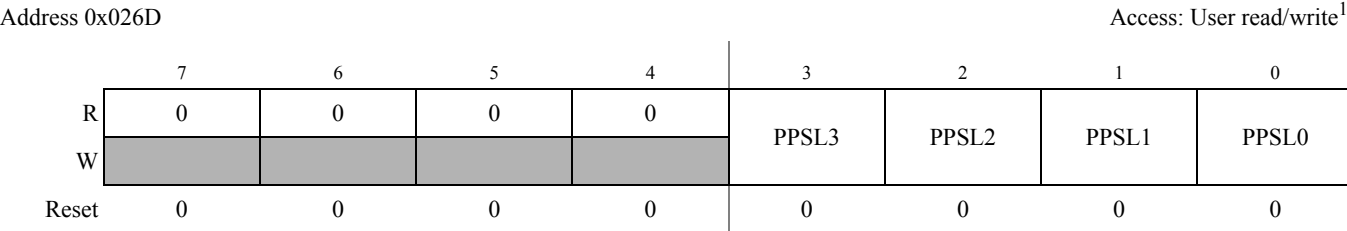
Figure 2-53. Port L Polarity Select Register (PPSL)
