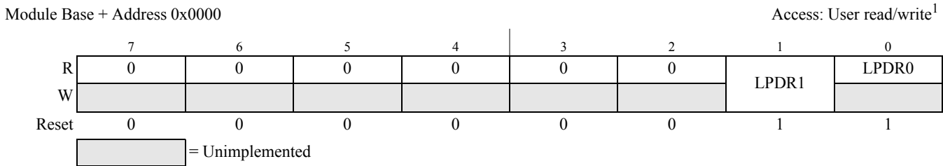
Figure 16-3. Port LP Data Register (LPDR)
