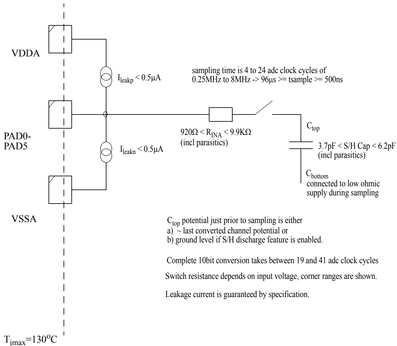
Figure C-2. ATD Input Parasitics
