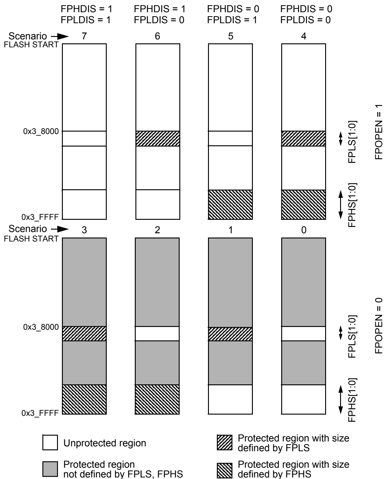
Figure 18-13. P-Flash Protection Scenarios
