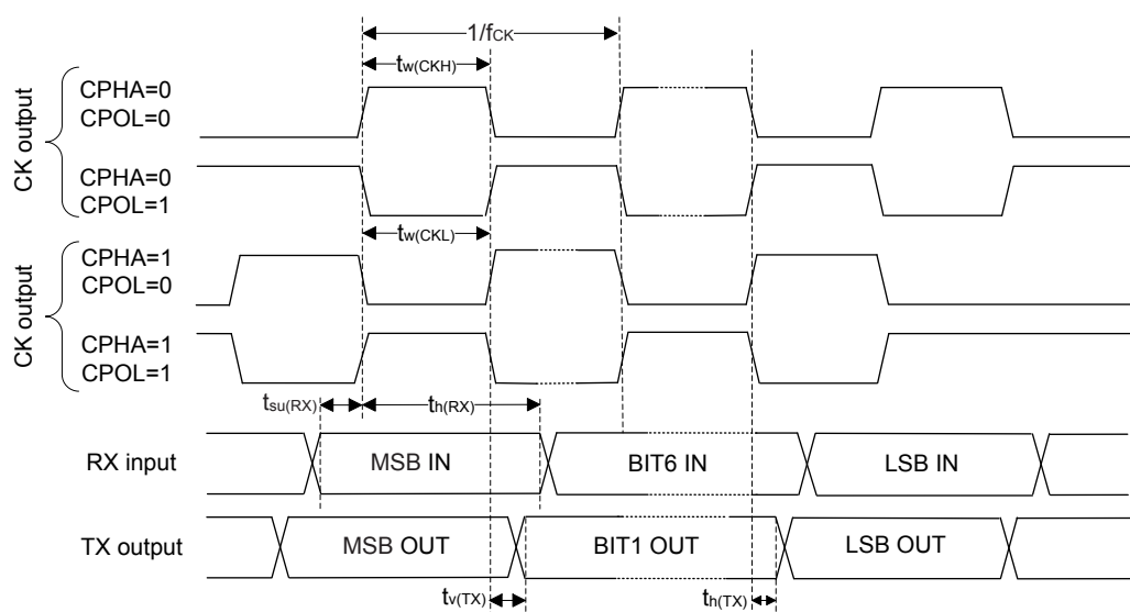
Figure 60. USART timing diagram in SPI master mode
