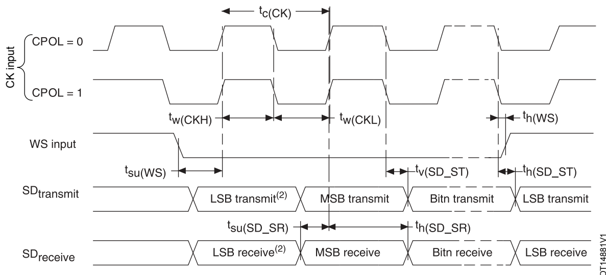
Figure 50. I2S slave timing diagram (Philips protocol)
