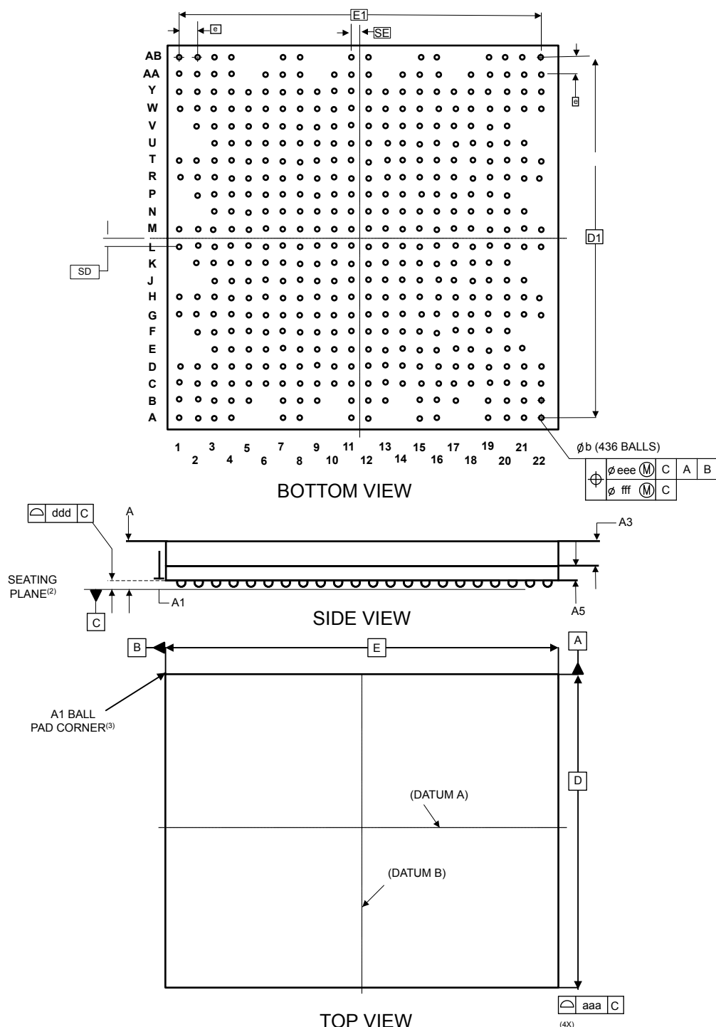
Figure 66. TFBGA436 - Outline
