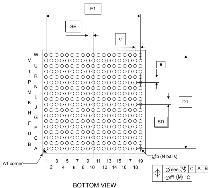
Figure 64. VFBGA361 - Outline
