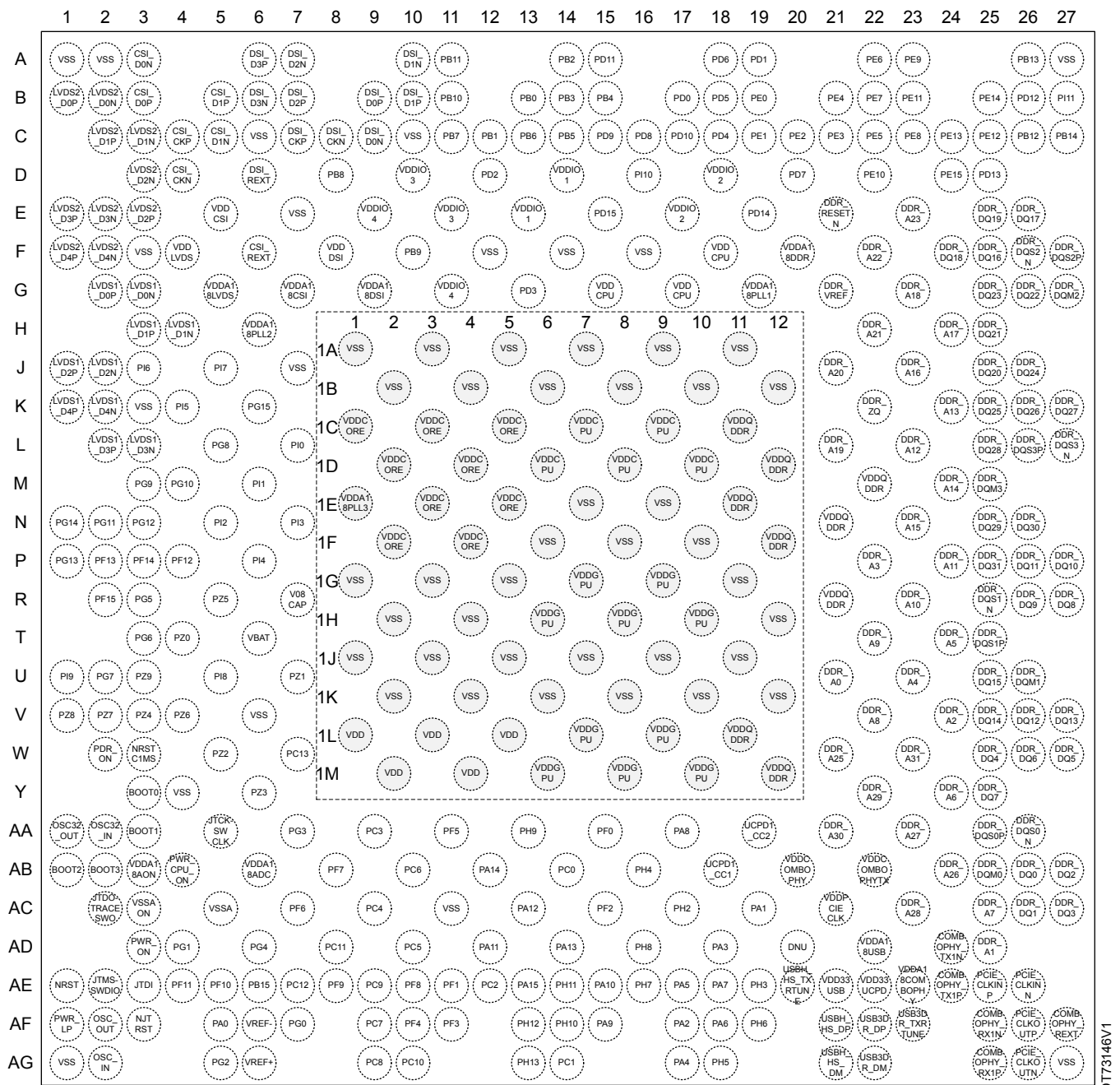
Figure 7. STM32MP25xC/F VFBGA424 pinout
