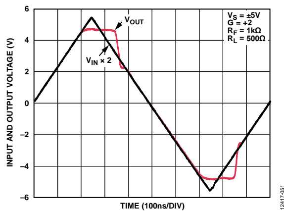
Figure 44. Output Overdrive Recovery (M1 Only)
