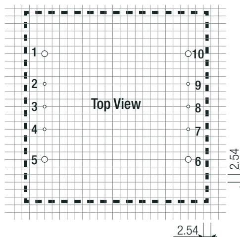
Recommended Footprint Details
