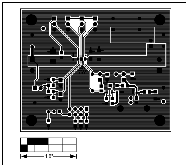
Figure 3. MAX14588 EV Kit PCB Layout—Component Side
