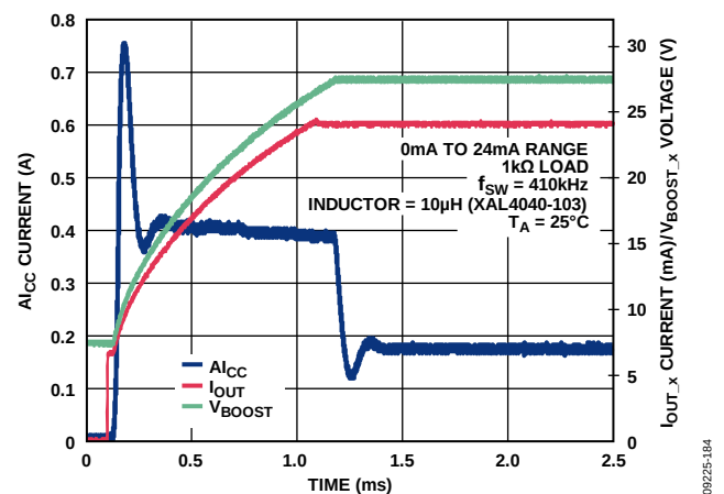
Figure 59. \text{AI}_{\text{CC}} Current vs. Time for 24 mA Step Through 1 k \Omega Load with Internal Compensation Resistor
